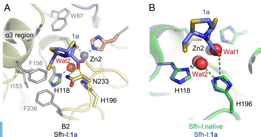
Fig. 5. 1a binding to Sfh-I and concomitant active-site conformational changes. Active-site zinc ions (gray spheres) and water molecules (red spheres) are labeled. (A) 1a (blue) bound in the active site of B2 Sfh-I (main chain colored as in Fig. 1). Hydrophobic residues, on the \alpha 3 region and within the active site, involved in binding 1a are shown as gray sticks. The 1a carboxylate bridges N233 and H196 (sticks). Residues involved in binding the active-site zinc ion (Zn2, gray sphere) and water (Wat2, red sphere) are represented as sticks. Interactions of 1a with the protein main chain or Zn2 are shown as yellow dashes. Protein–zinc and protein–water interactions are shown as gray dashes. (B) Superposition of Sfh-I:1a (blue) with unliganded, native Sfh-I (PDB ID code 3SD9, green). Interactions of H118 and H196 with the BTZ or Wat2 are shown as dashes.
