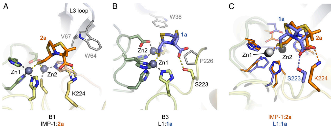
Fig. 4. L-bisthiazolidine binding to B1 (IMP-1) and B3 (L1) metallo- \beta -lactamases. Close-up view of IMP-1 and L1 active sites with bound L-BTZ (sticks, colored as in Fig. 2). Protein main chain is colored from the N (light blue) to C terminus (light red). Residues that interact with the zinc ions (Zn1 and Zn2, gray spheres) are shown as sticks (colored as main chain), whereas hydrophobic residues that stabilize BTZ binding are shown as gray sticks. IMP-1 K224 and L1 S223 (labeled) interact with the BTZ carboxylate. (A) 2a bound to B1 IMP-1. Protein–zinc interactions are shown as gray dashes and BTZ–protein or BTZ–zinc interactions are shown as yellow dashes. (B) 1a bound to B3 L1. Interactions shown as in A. (C) Superposition of IMP-1:2a (orange) and L1:1a (blue). BTZ–protein or BTZ–zinc interactions are shown as dashes colored orange (IMP-1:2a) or blue (L1:1a).
